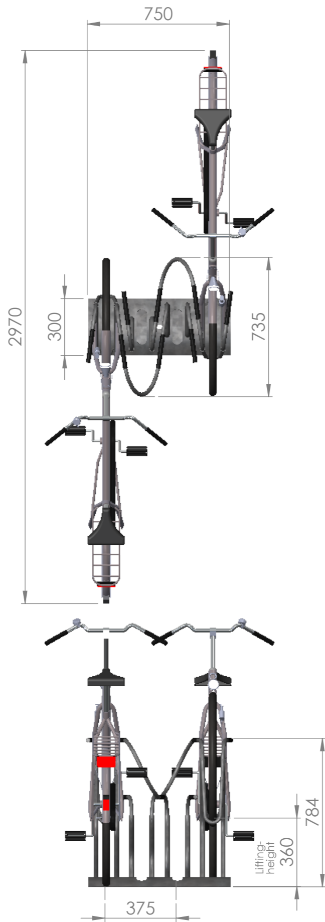
K1512, Cobra 4D double-sided - h.2.h. 375 mm
